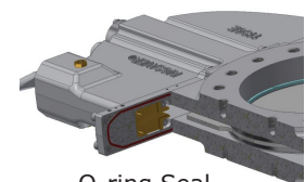
O-ring Seal
